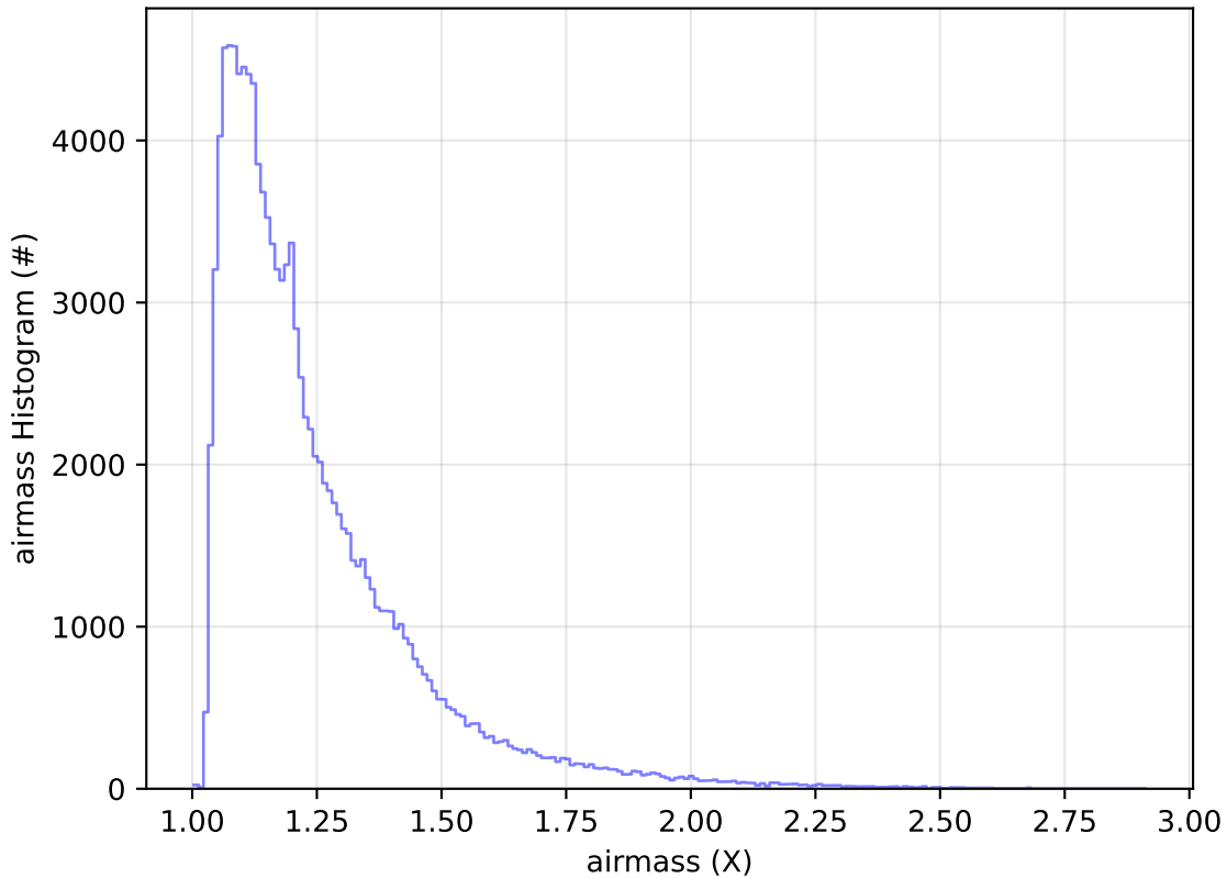
ddf_acor_sf10_lsf40_lsr20_v3.4_10yrs All sky u band: airmass Histogram
