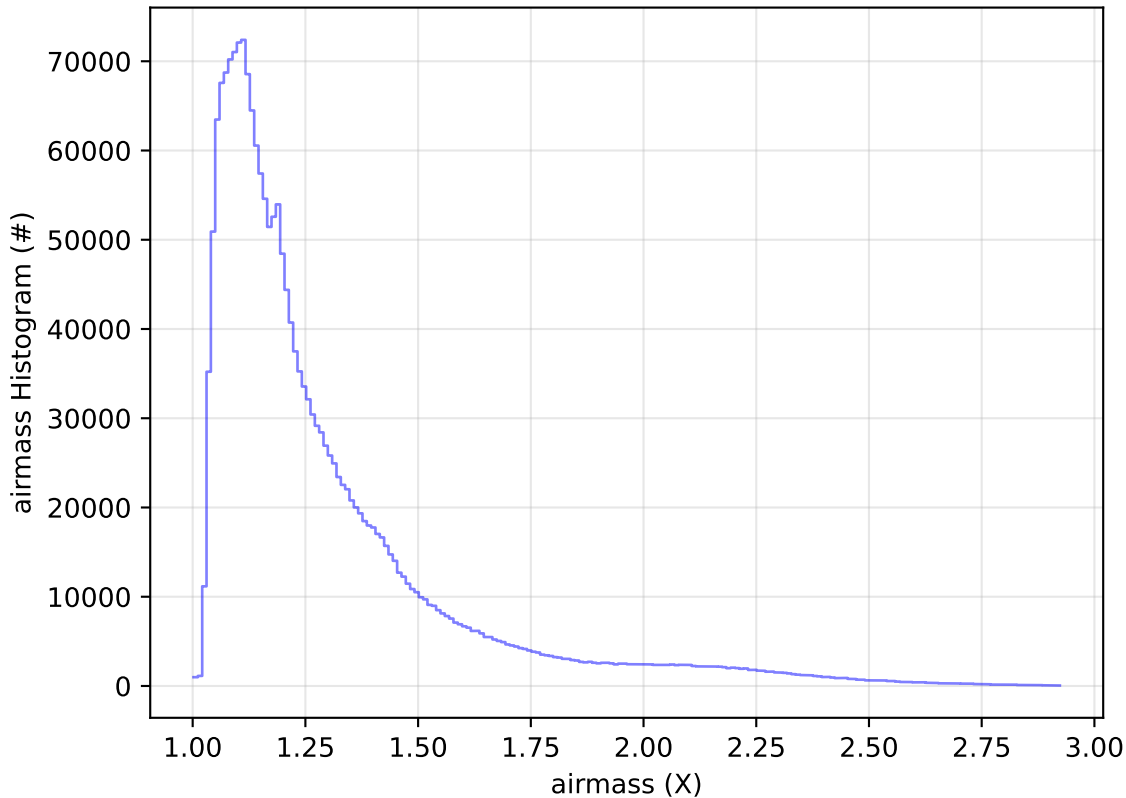
ddf_acor_sf10_lsf40_lsr20_v3.4_10yrs All sky all bands: airmass Histogram
