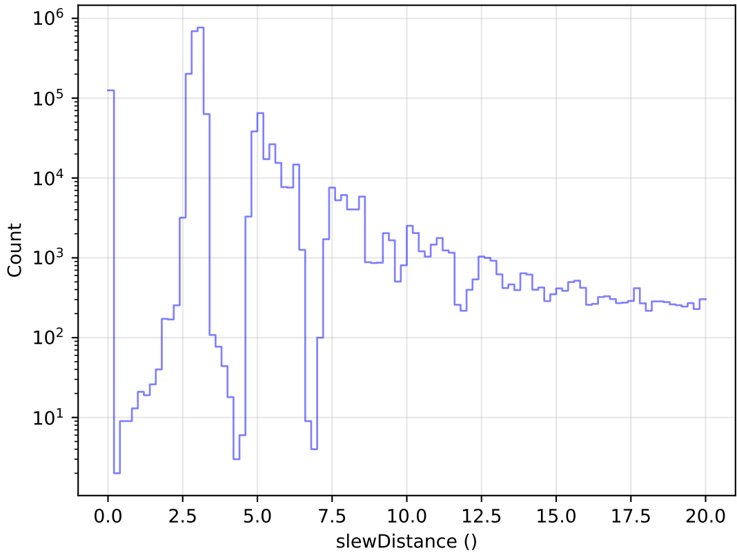
ddf_acor_sf10_lsf40_lsr20_v3.4_10yrs All visits: Zoom Slew Distance Histogram
