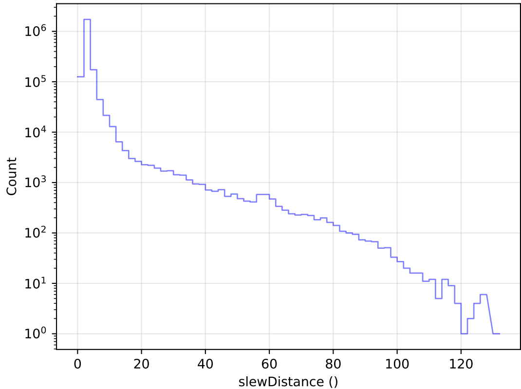
ddf_acor_sf10_lsf40_lsr20_v3.4_10yrs All visits: Slew Distance Histogram
