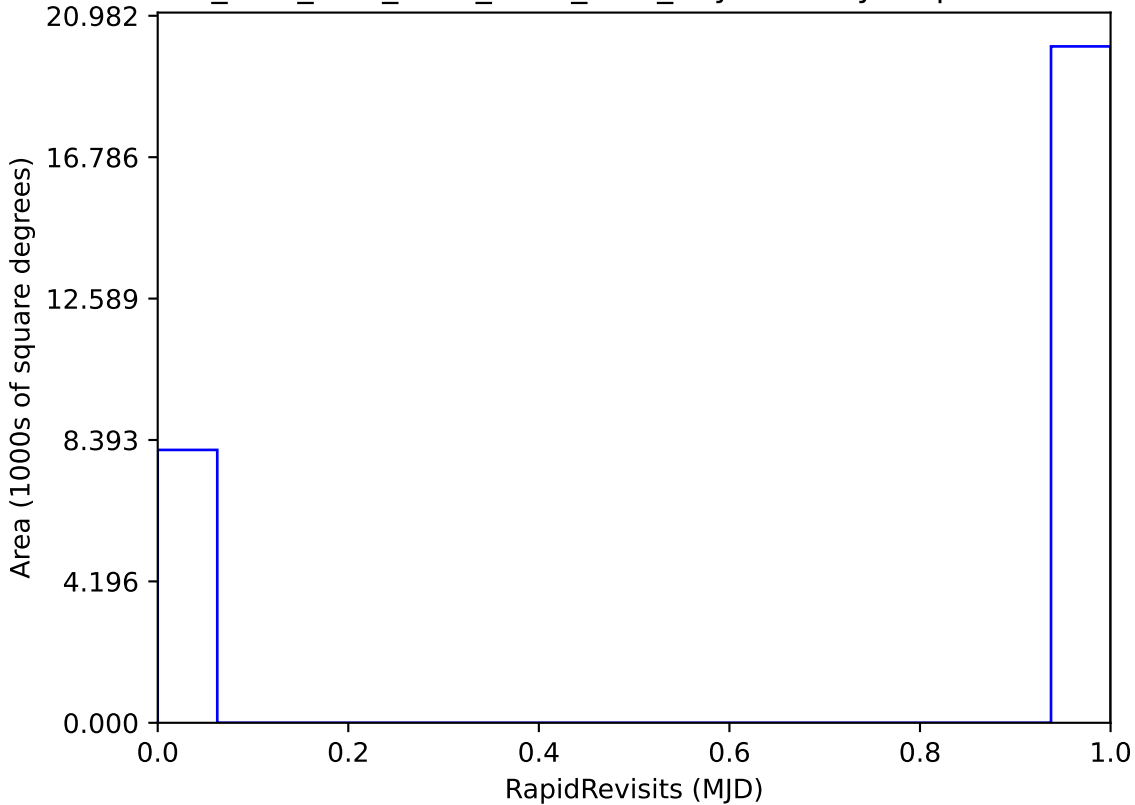
ddf_acor_sf10_lsf40_lsr20_v3.4_10yrs All sky: RapidRevisits
