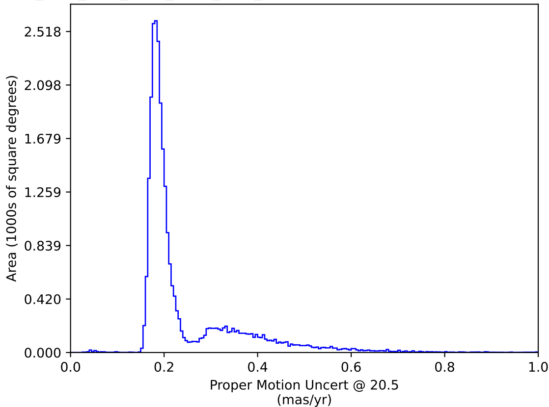
ddf_acor_sf10_lsf40_lsr20_v3.4_10yrs All sky: Proper Motion Uncert @ 20.5
