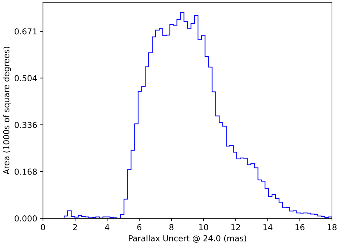
ddf_acor_sf10_lsf40_lsr20_v3.4_10yrs WFD: Parallax Uncert @ 24.0
