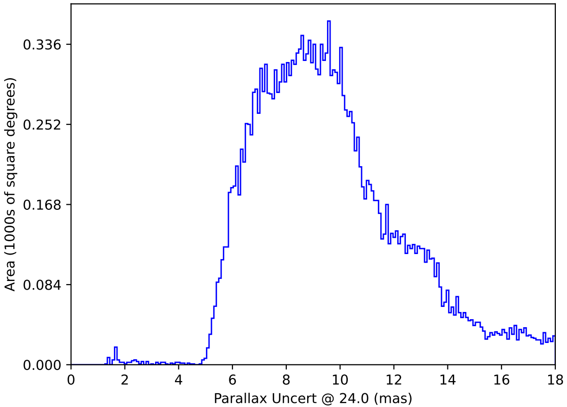
ddf_acor_sf10_lsf40_lsr20_v3.4_10yrs All sky: Parallax Uncert @ 24.0
