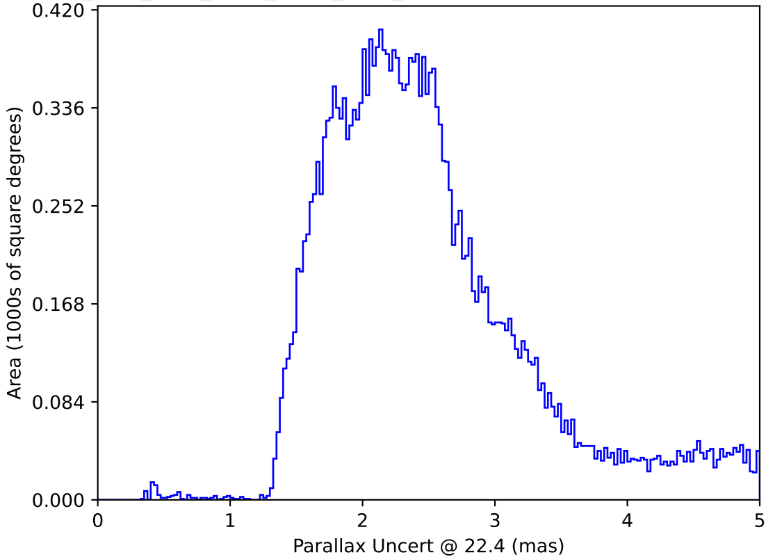
ddf_acor_sf10_lsf40_lsr20_v3.4_10yrs All sky: Parallax Uncert @ 22.4
