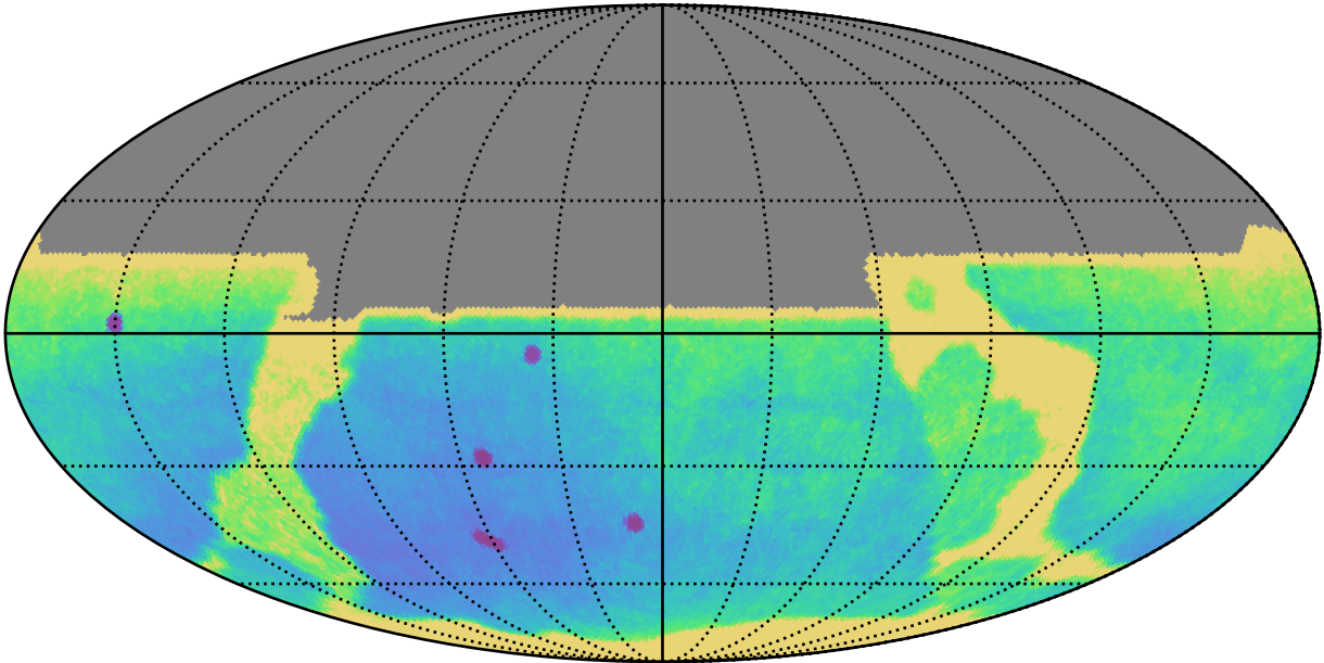
ddf_acor_sf10_lsf40_lsr20_v3.4_10yrs All sky y band only: Parallax Uncert @ 21.3
