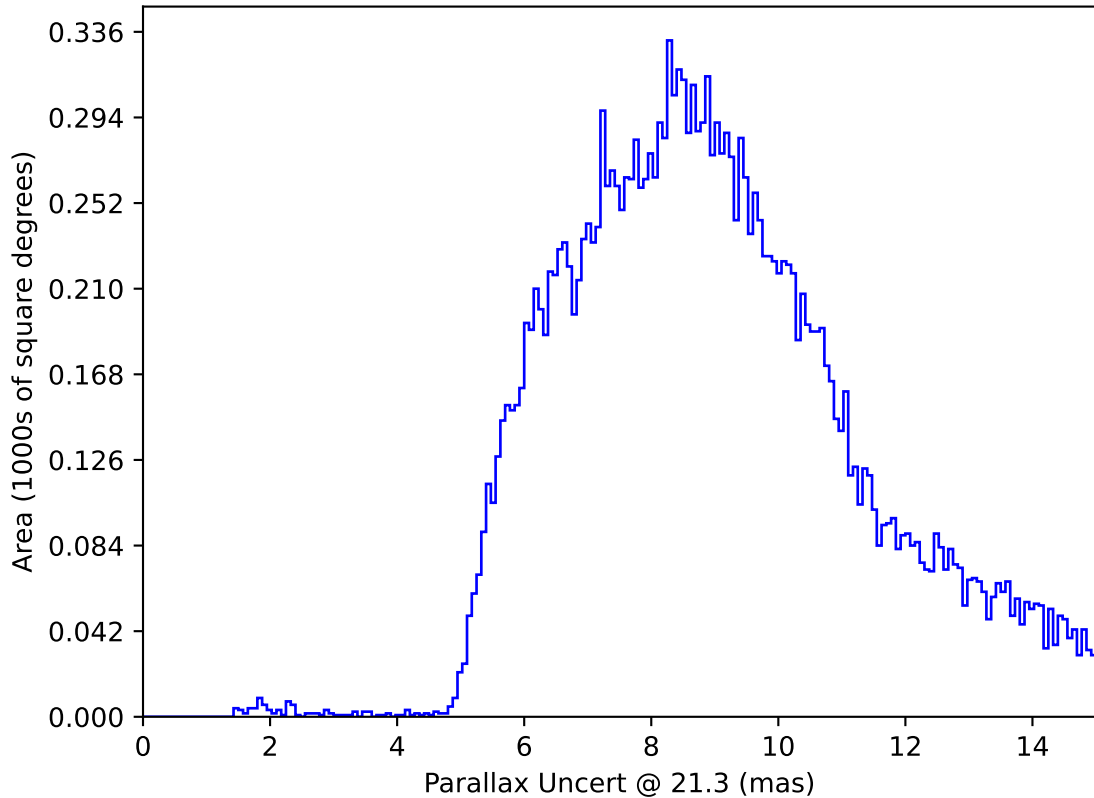
ddf_acor_sf10_lsf40_lsr20_v3.4_10yrs All sky y band only: Parallax Uncert @ 21.3
