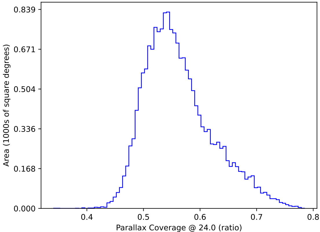
ddf_acor_sf10_lsf40_lsr20_v3.4_10yrs WFD: Parallax Coverage @ 24.0
