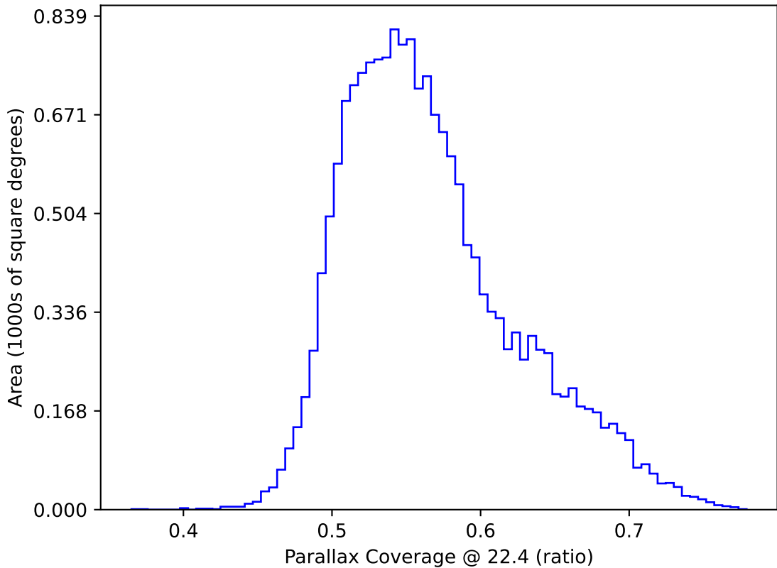
ddf_acor_sf10_lsf40_lsr20_v3.4_10yrs WFD: Parallax Coverage @ 22.4
