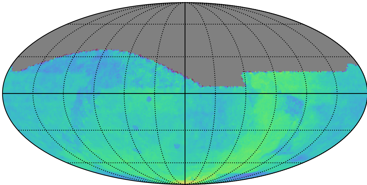
ddf_acor_sf10_lsf40_lsr20_v3.4_10yrs All sky: Parallax Coverage @ 22.4
