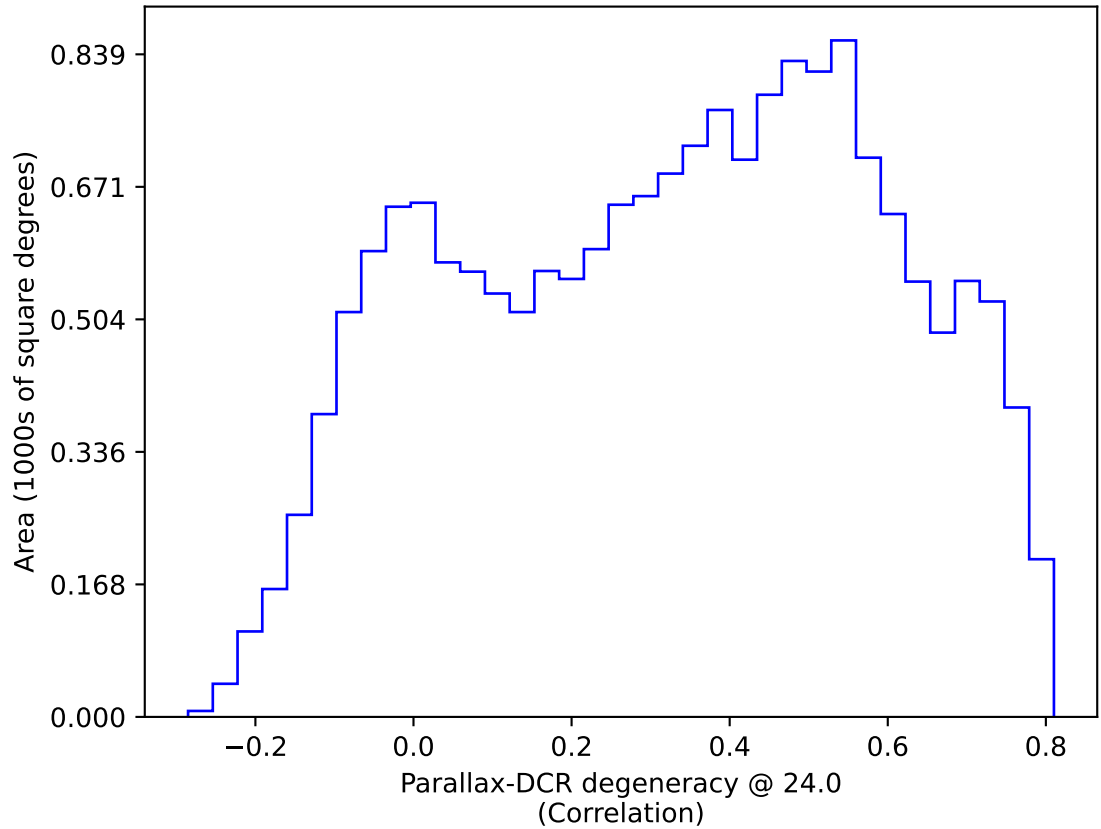
ddf_acor_sf10_lsf40_lsr20_v3.4_10yrs WFD: Parallax-DCR degeneracy @ 24.0
