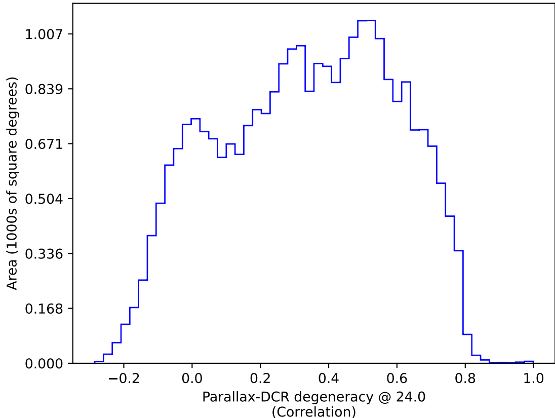
ddf_acor_sf10_ls40_lsr20_v3.4_10yrs All sky: Parallax-DCR degeneracy @ 24.0
