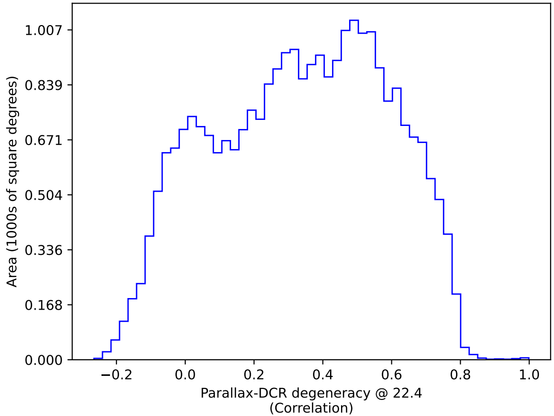
ddf_acor_sf10_ls40_lsr20_v3.4_10yrs All sky: Parallax-DCR degeneracy @ 22.4
