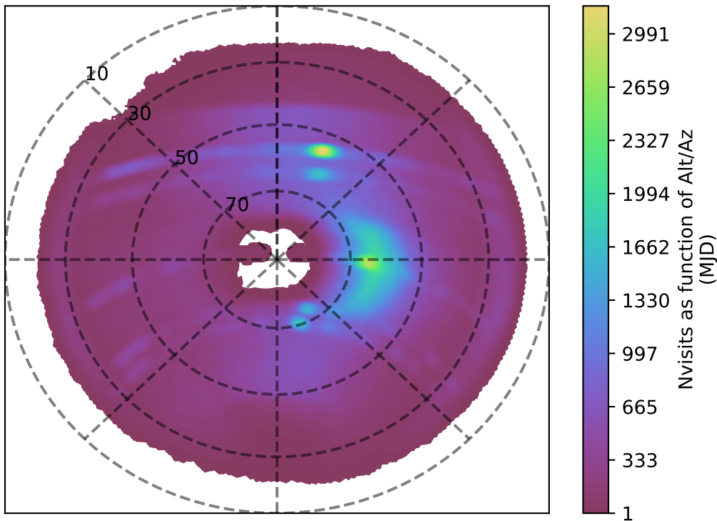
ddf_acor_sf10_lsf40_lsr20_v3.4_10yrs z band: Nvisits as function of Alt/Az
