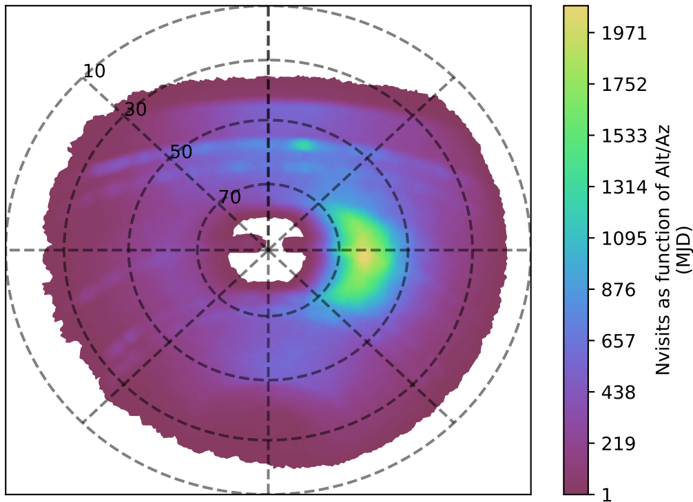
ddf_acor_sf10_lsf40_lsr20_v3.4_10yrs y band: Nvisits as function of Alt/Az
