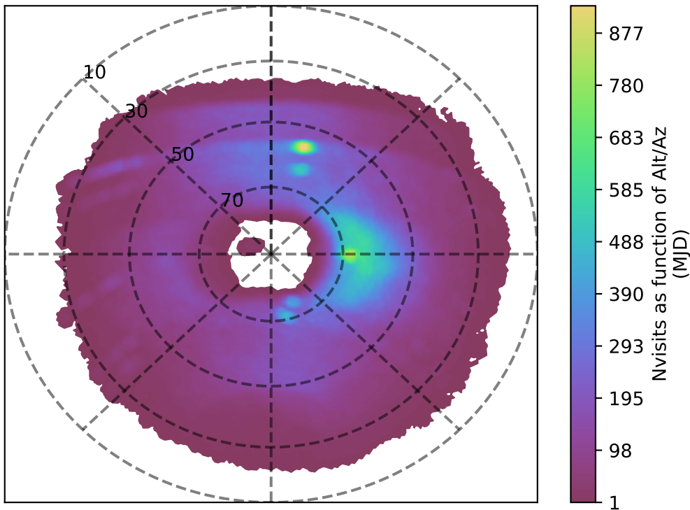
ddf_acor_sf10_lsf40_lsr20_v3.4_10yrs u band: Nvisits as function of Alt/Az
