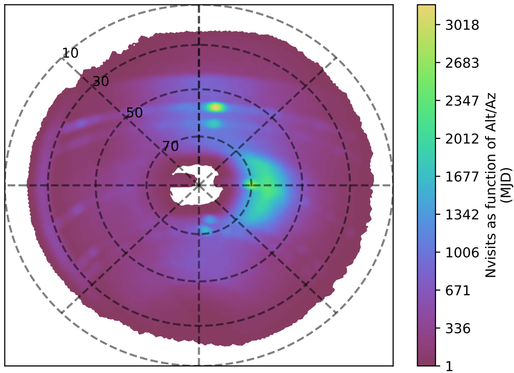
ddf_acor_sf10_lsf40_lsr20_v3.4_10yrs r band: Nvisits as function of Alt/Az
