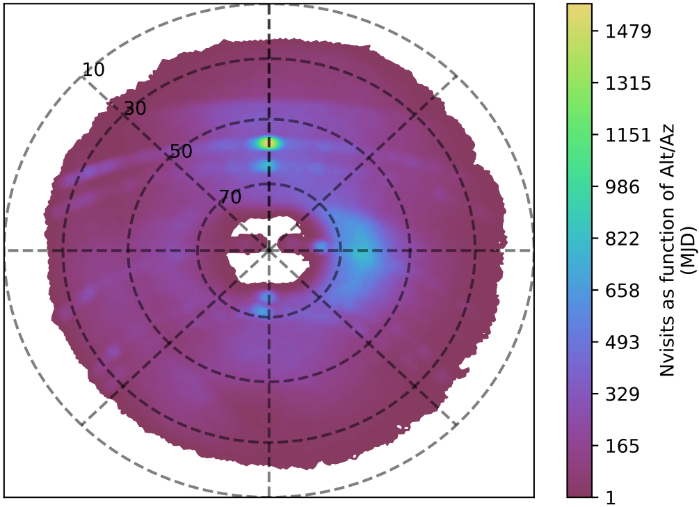
ddf_acor_sf10_lsf40_lsr20_v3.4_10yrs g band: Nvisits as function of Alt/Az
