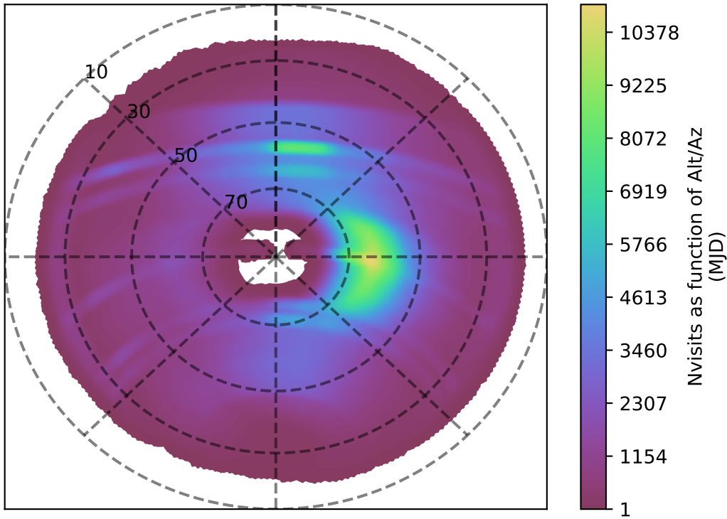
ddf_acor_sf10_ls40_lsr20_v3.4_10yrs all bands: Nvisits as function of Alt/Az
