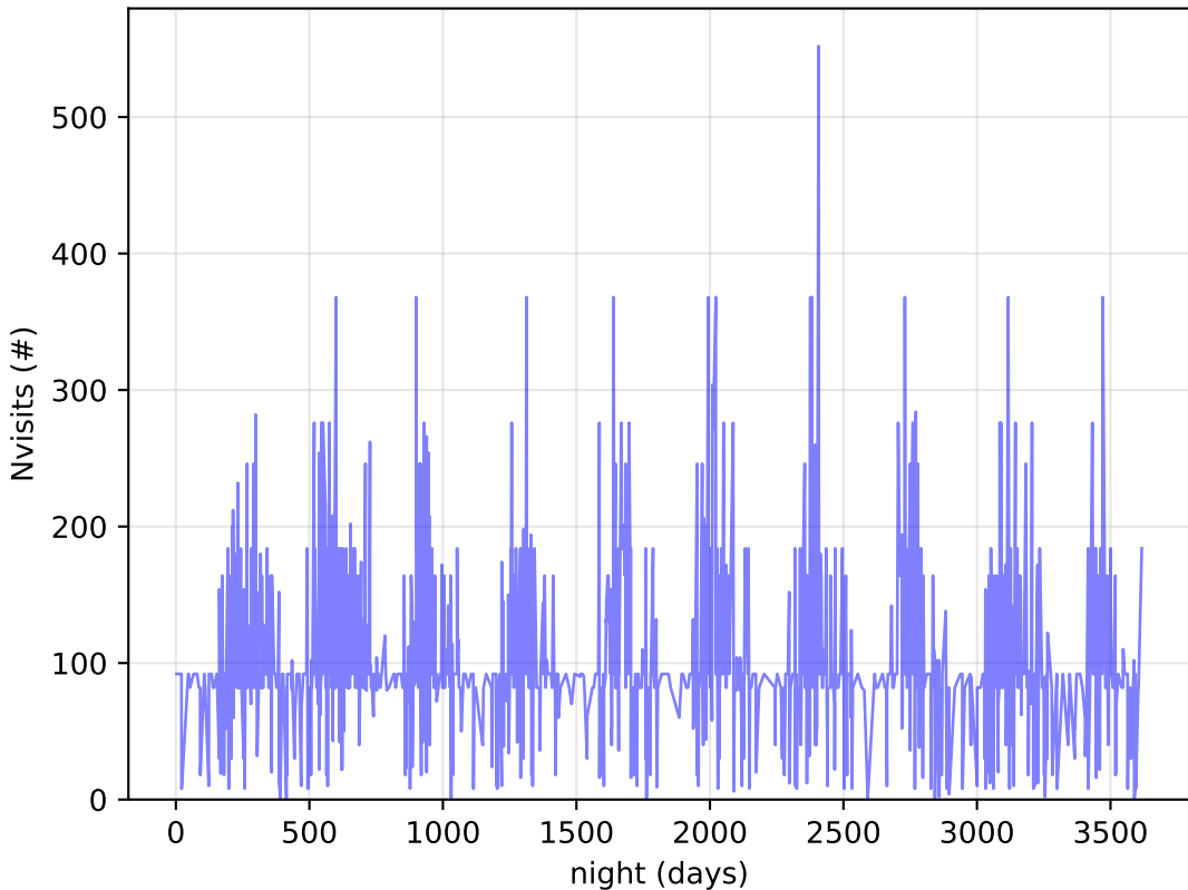
ddf_acor_sf10_ls40_lsr20_v3.4_10yrs DDF: Nvisits
