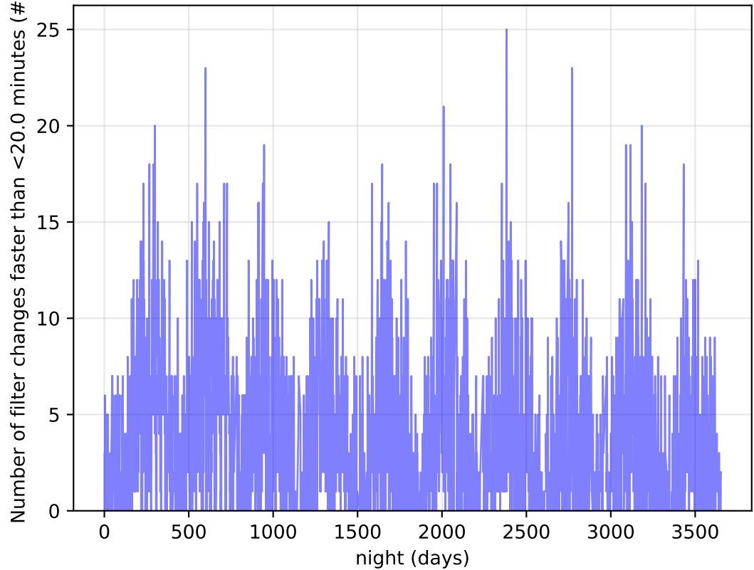
ddf_acor_sf10_Isf40_Isr20_v3.4_10yrs Per Night: Number of filter changes faster than <20.0 minutes
