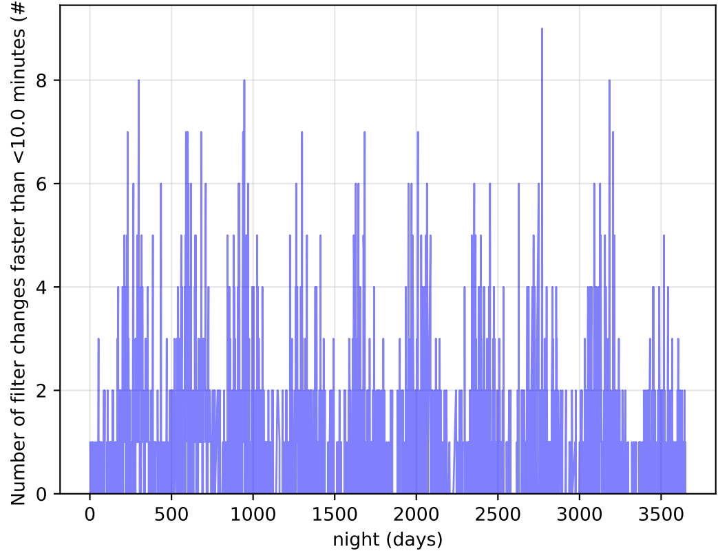
ddf_acor_sf10_Isf40_Isr20_v3.4_10yrs Per Night: Number of filter changes faster than <10.0 minutes
