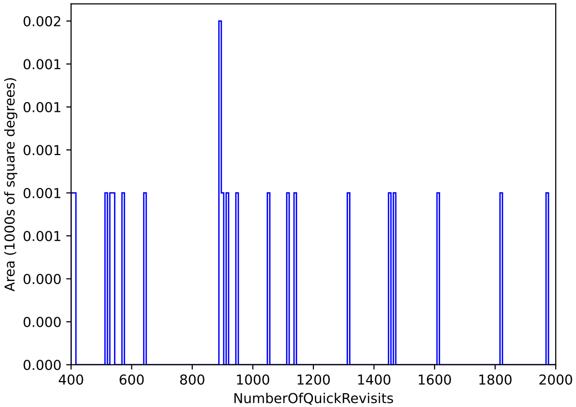
ddf_acor_sf10_lsf40_lsr20_v3.4_10yrs WFD: NumberOfQuickRevisits
