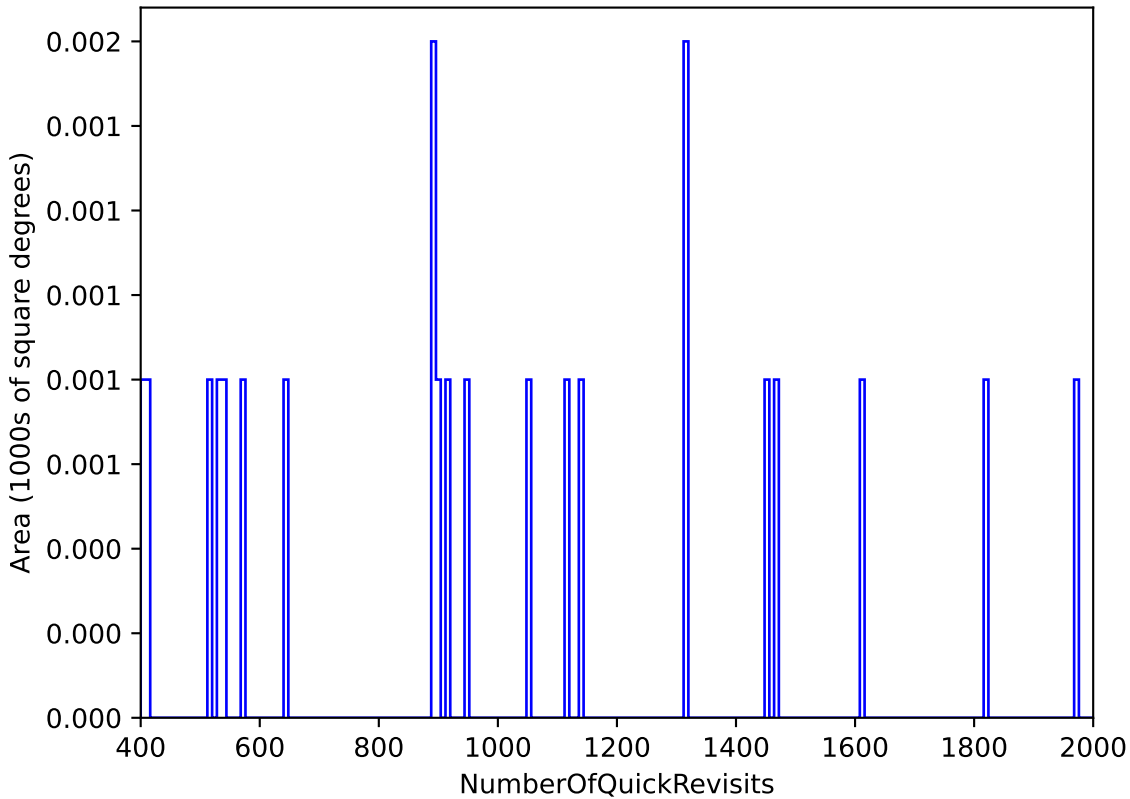
ddf_acor_sf10_lsf40_lsr20_v3.4_10yrs All sky: NumberOfQuickRevisits
