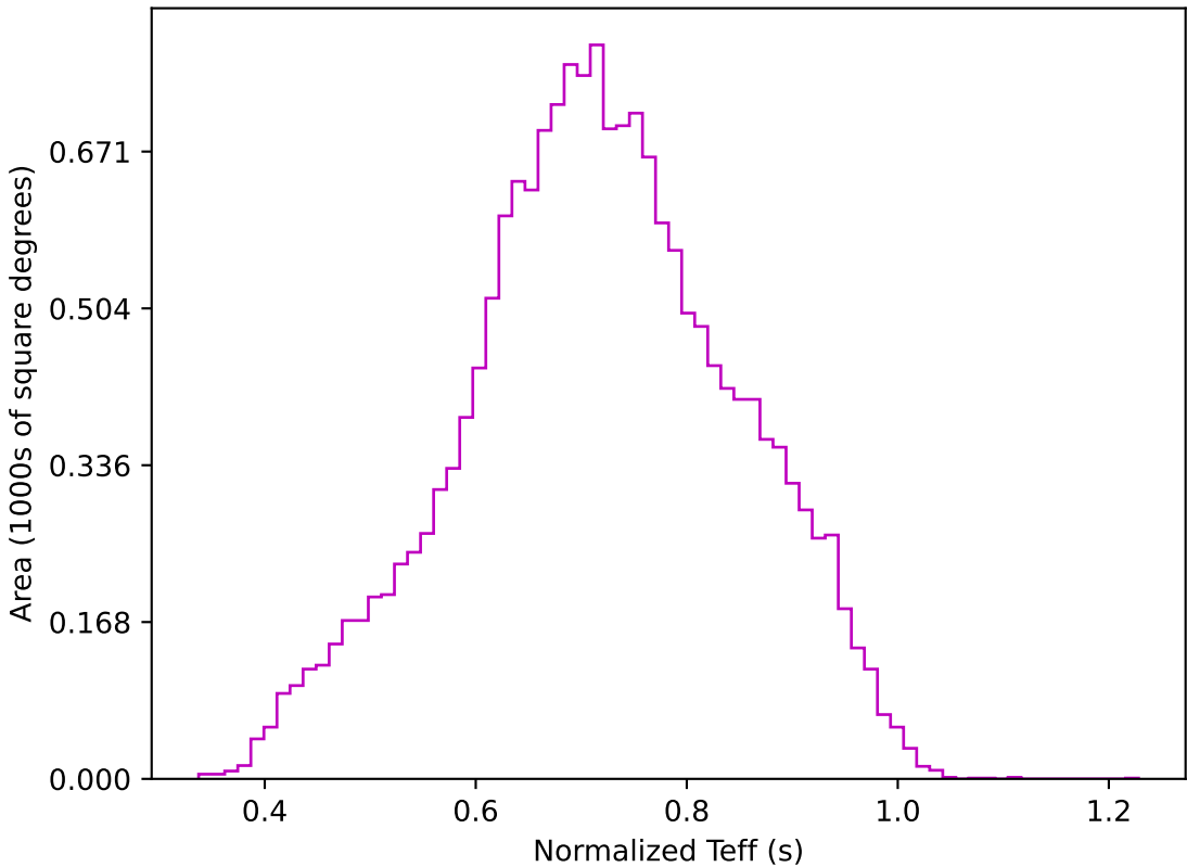
ddf_acor_sf10_lsf40_lsr20_v3.4_10yrs WFD z band: Normalized Teff
