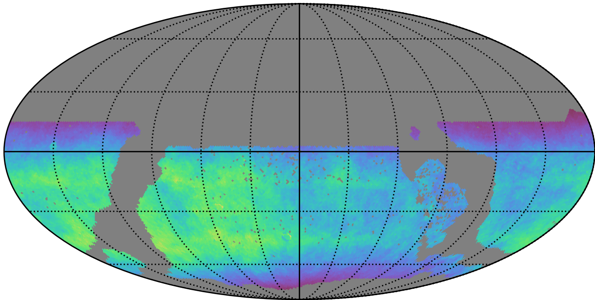
ddf_acor_sf10_lsf40_lsr20_v3.4_10yrs WFD y band: Normalized Teff
