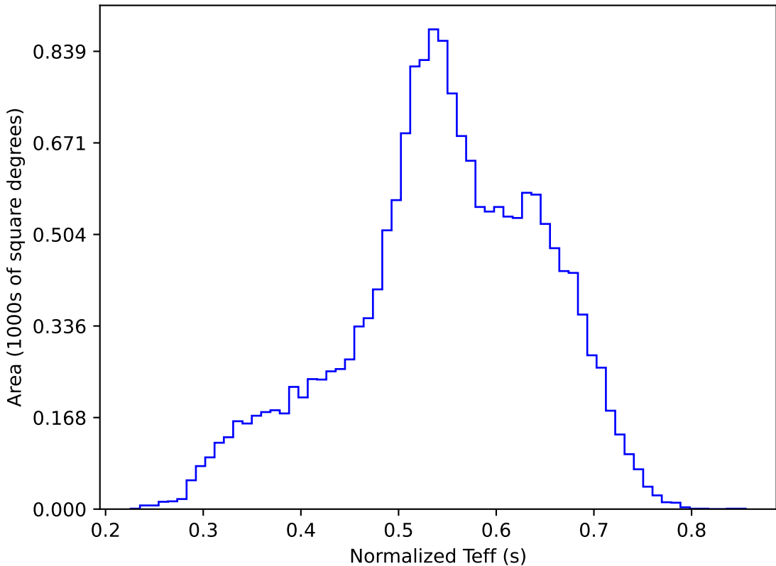
ddf_acor_sf10_lsf40_lsr20_v3.4_10yrs WFD y band: Normalized Teff
