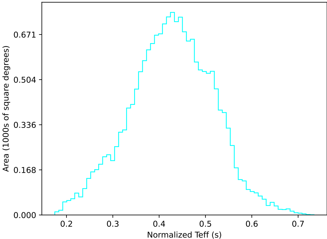
ddf_acor_sf10_lsf40_lsr20_v3.4_10yrs WFD u band: Normalized Teff
