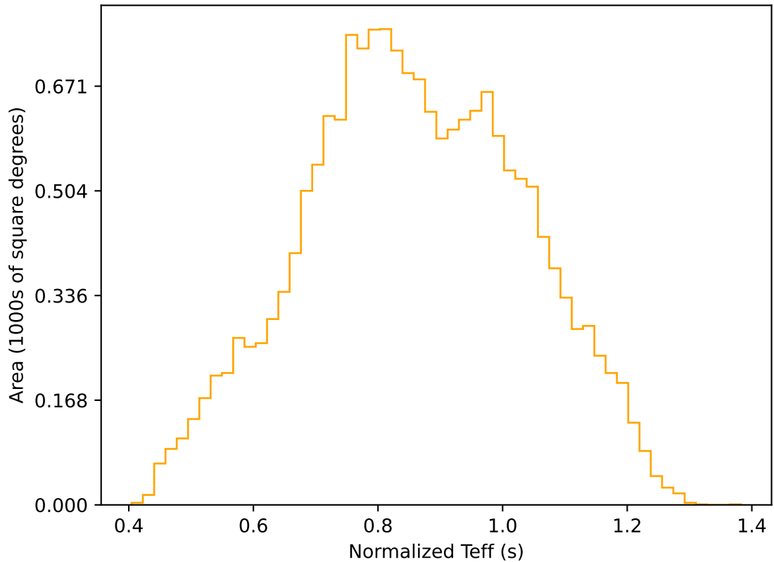
ddf_acor_sf10_lsf40_lsr20_v3.4_10yrs WFD r band: Normalized Teff
