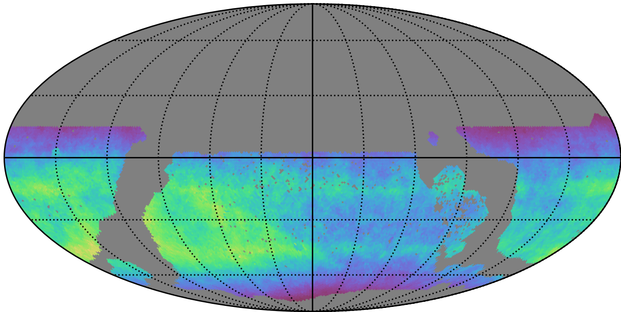
ddf_acor_sf10_lsf40_lsr20_v3.4_10yrs WFD i band: Normalized Teff
