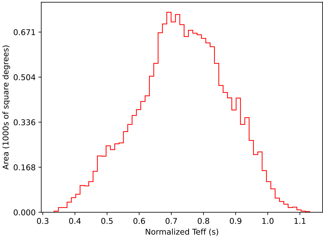
ddf_acor_sf10_lsf40_lsr20_v3.4_10yrs WFD i band: Normalized Teff
