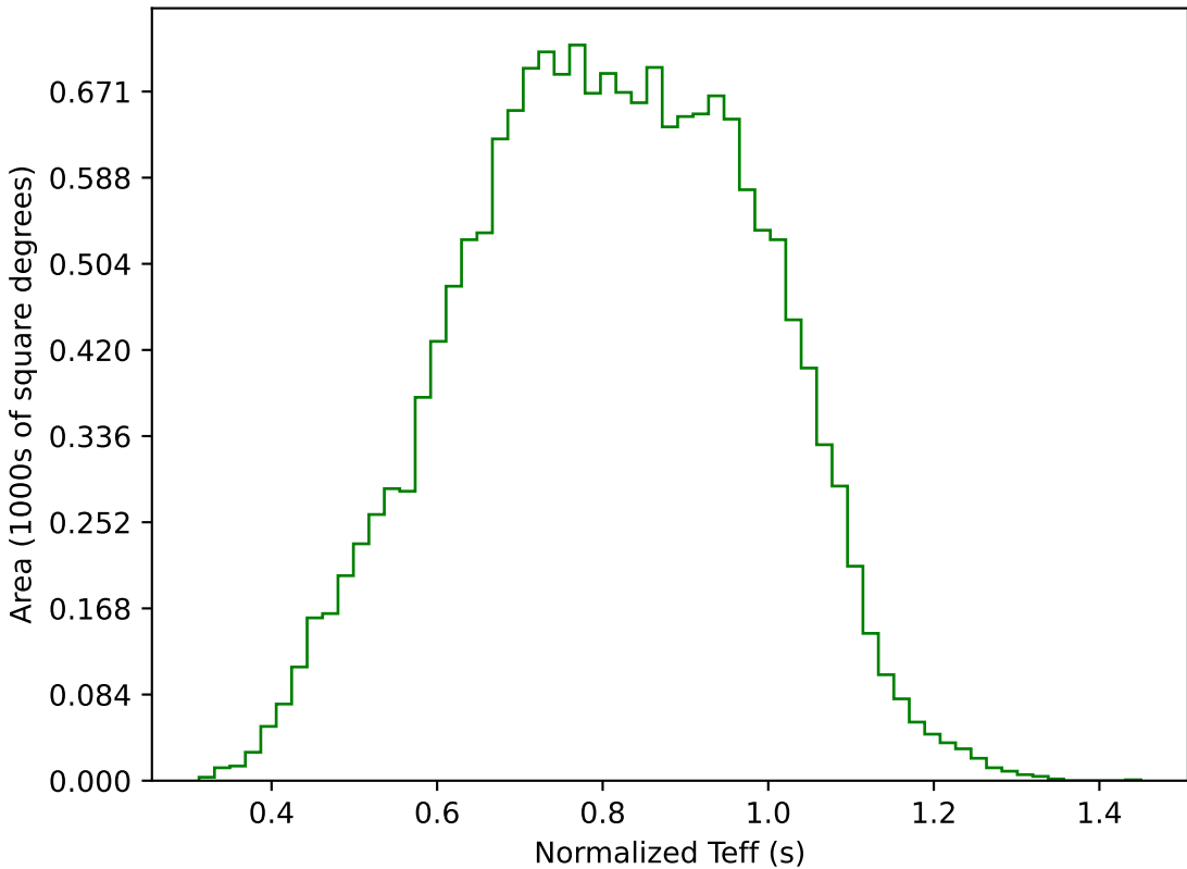
ddf_acor_sf10_lsf40_lsr20_v3.4_10yrs WFD g band: Normalized Teff
