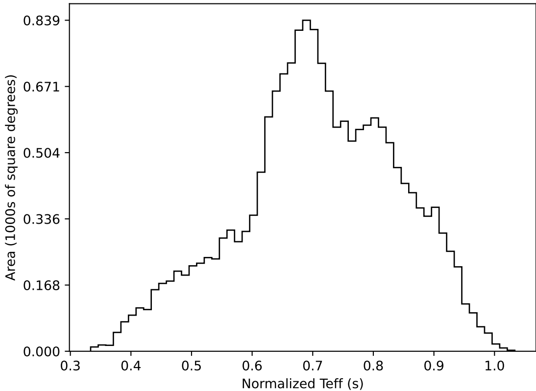
ddf_acor_sf10_lsf40_lsr20_v3.4_10yrs WFD all bands: Normalized Teff
