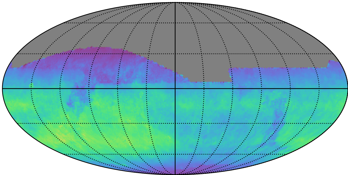
ddf_acor_sf10_lsf40_lsr20_v3.4_10yrs All sky z band: Normalized Teff
