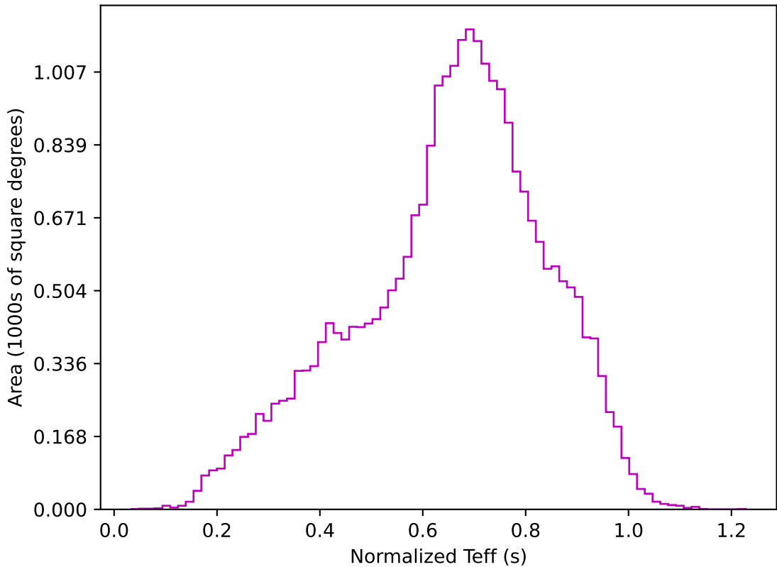
ddf_acor_sf10_lsf40_lsr20_v3.4_10yrs All sky z band: Normalized Teff
