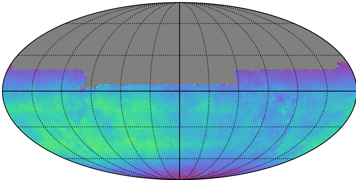
ddf_acor_sf10_lsf40_lsr20_v3.4_10yrs All sky y band: Normalized Teff
