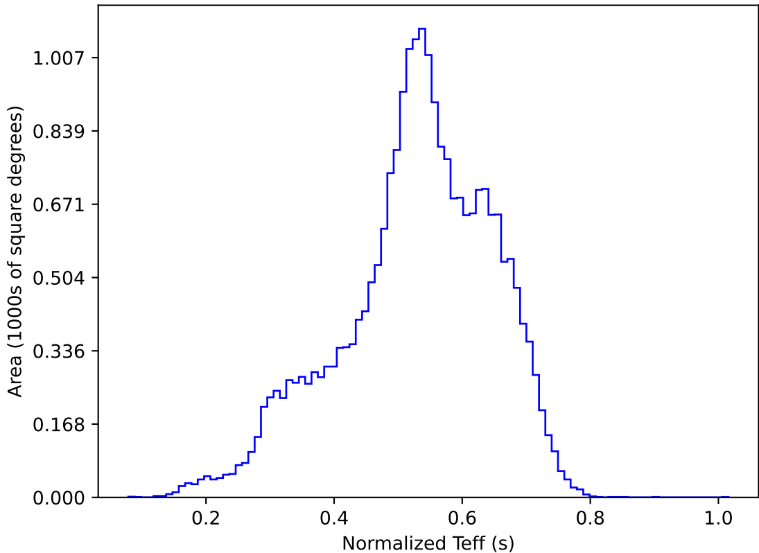
ddf_acor_sf10_lsf40_lsr20_v3.4_10yrs All sky y band: Normalized Teff
