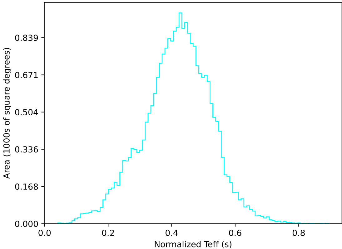
ddf_acor_sf10_lsf40_lsr20_v3.4_10yrs All sky u band: Normalized Teff
