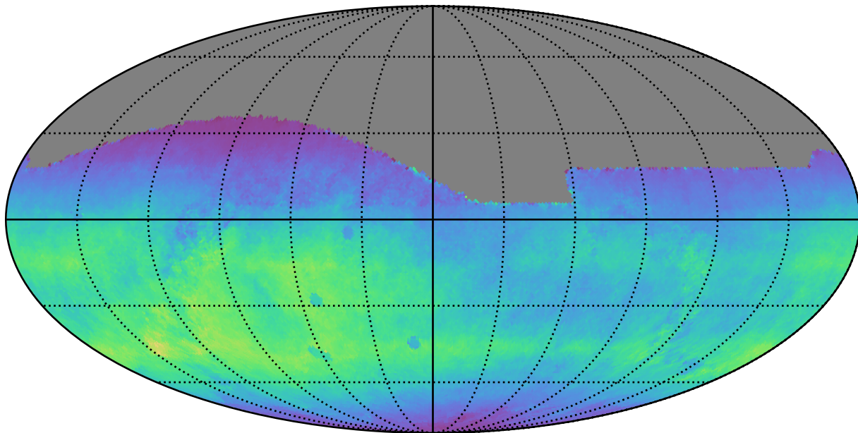
ddf_acor_sf10_lsf40_lsr20_v3.4_10yrs All sky r band: Normalized Teff
