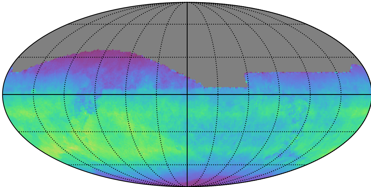
ddf_acor_sf10_lsf40_lsr20_v3.4_10yrs All sky i band: Normalized Teff
