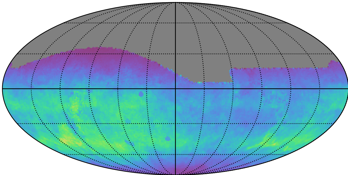
ddf_acor_sf10_lsf40_lsr20_v3.4_10yrs All sky g band: Normalized Teff
