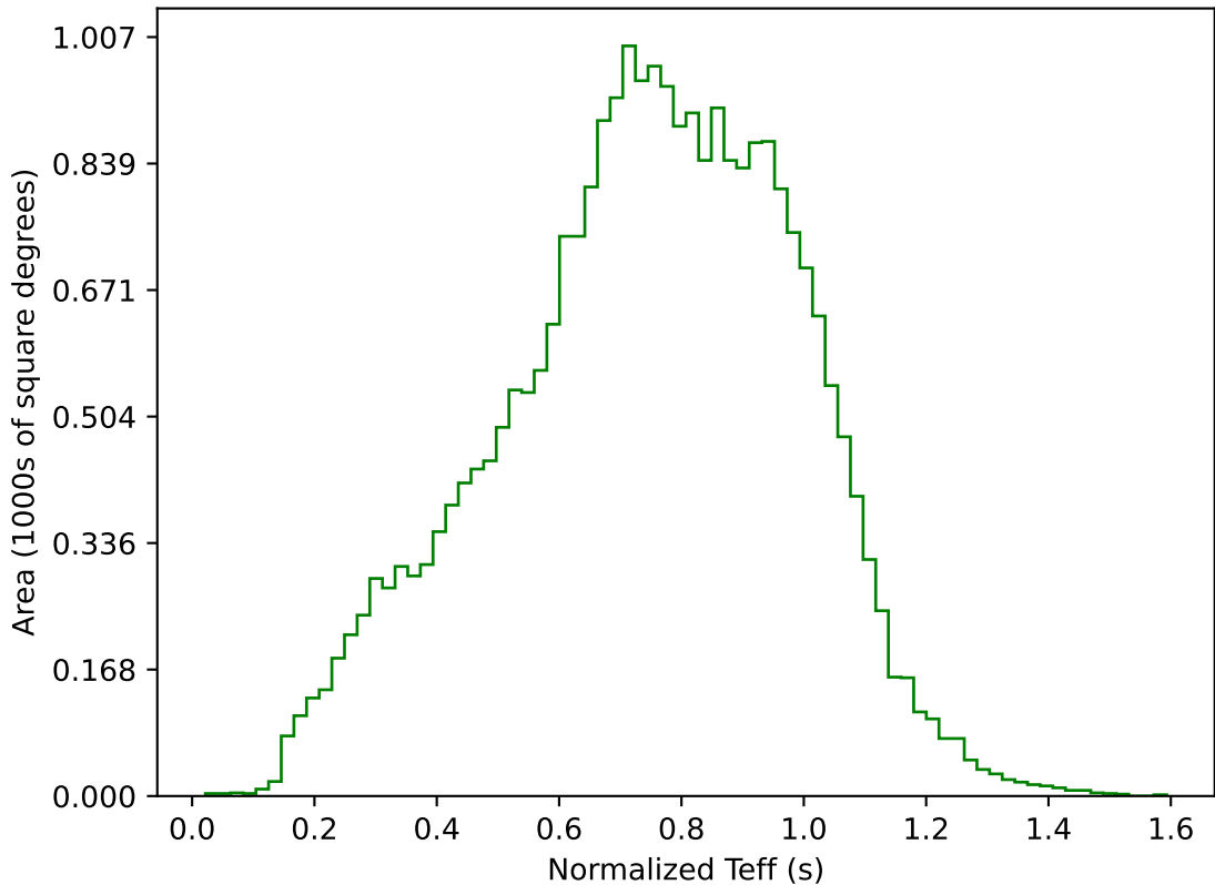
ddf_acor_sf10_lsf40_lsr20_v3.4_10yrs All sky g band: Normalized Teff
