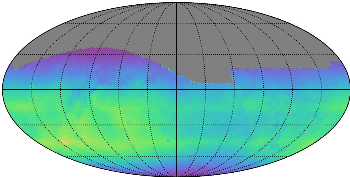
ddf_acor_sf10_lsf40_lsr20_v3.4_10yrs All sky all bands: Normalized Teff
