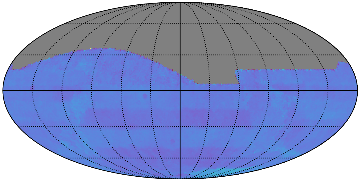
ddf_acor_sf10_lsf40_lsr20_v3.4_10yrs All sky: Normalized Proper Motion Uncert @ 24.0
