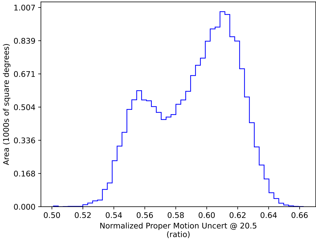
ddf_acor_sf10_lsf40_lsr20_v3.4_10yrs WFD: Normalized Proper Motion Uncert @ 20.5
