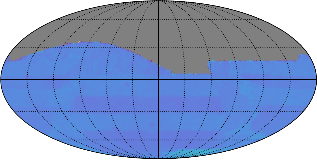
ddf_acor_sf10_lsf40_lsr20_v3.4_10yrs All sky: Normalized Proper Motion Uncert @ 20.5
